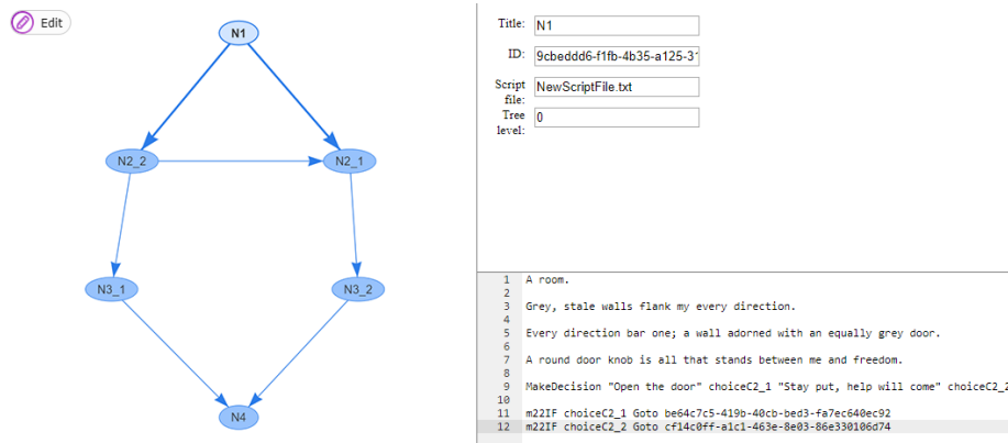
Fig. 1. Authoring tool's GUI (prototype version)
